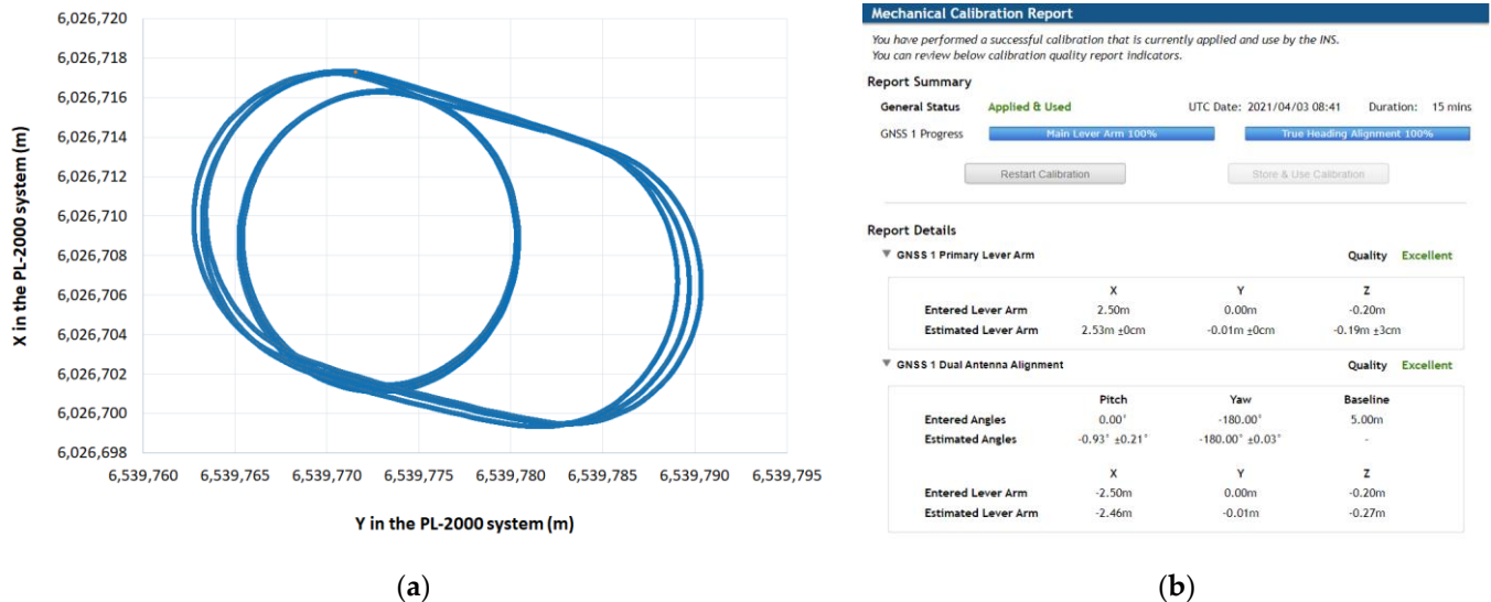
Figure 4. Melex movement trajectory (a) and the results of the Ekinox2-U system calibration (b) of 19 May 2021.
