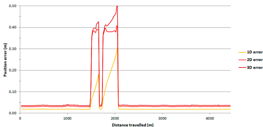
Figure 8. Variability of the 1D, 2D and 3D position errors recorded using the Ekinox2-U system in the RTK mode on route no. 1.
