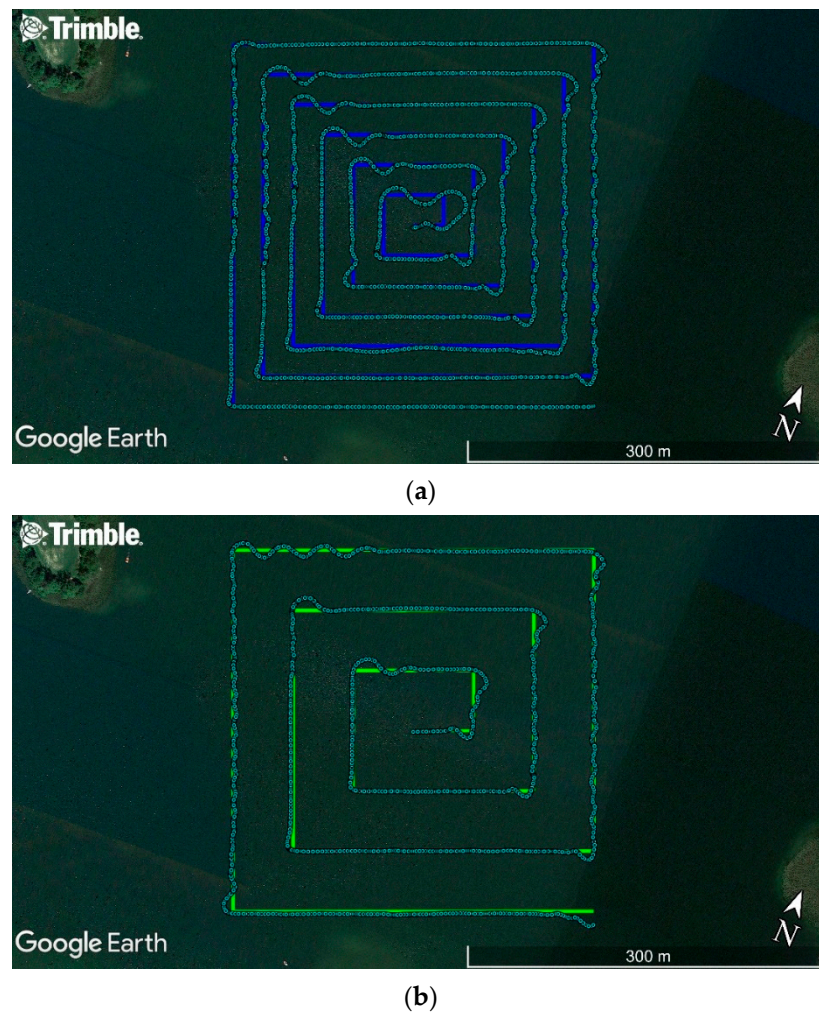
Figure 5. Arrangement of the route's sounding profiles—spiral every (a) 25 m and (b) 50 m, on which the ASV/USV moved during the hydrographic surveys. The “HydroDron” vessel's trajectory was marked with a sky-blue colour.
