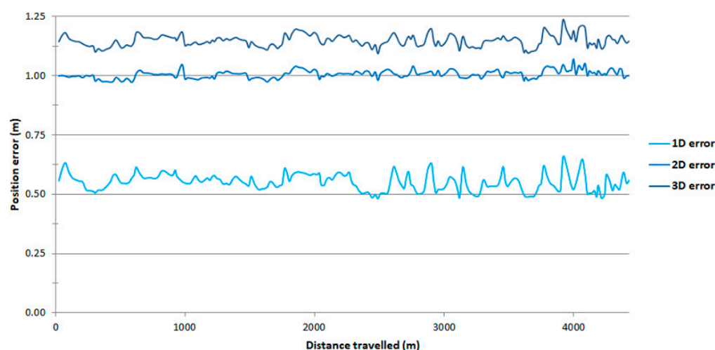
Figure 9. Variability of the 1D, 2D and 3D position errors recorded using the Ellipse-D system in the DGPS mode on route no. 1.
